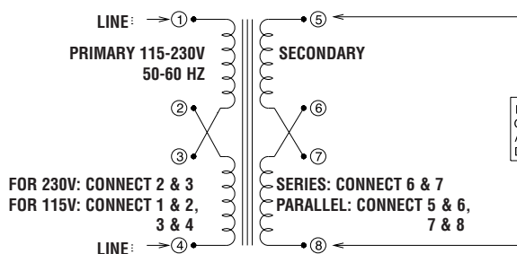
Schematic 1
