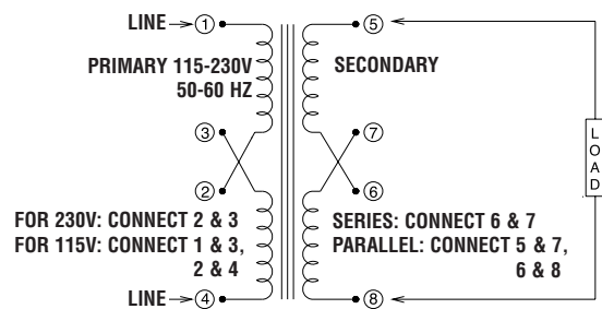
Schematic 2
